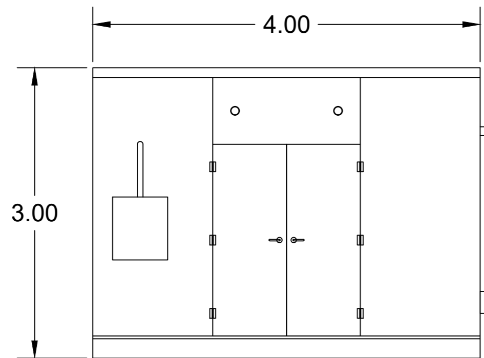
FRONT VIEW
